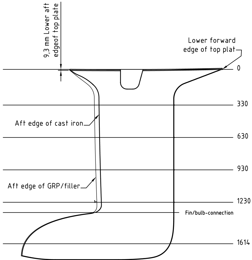
Principle of maximum templates for the X-35 keel Scale 1:5
